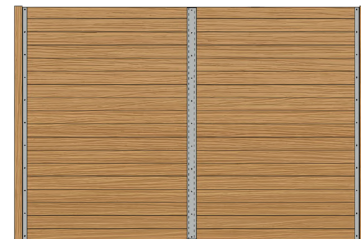
U-channel Solid
